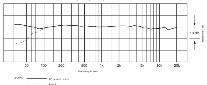
Frequency Response
